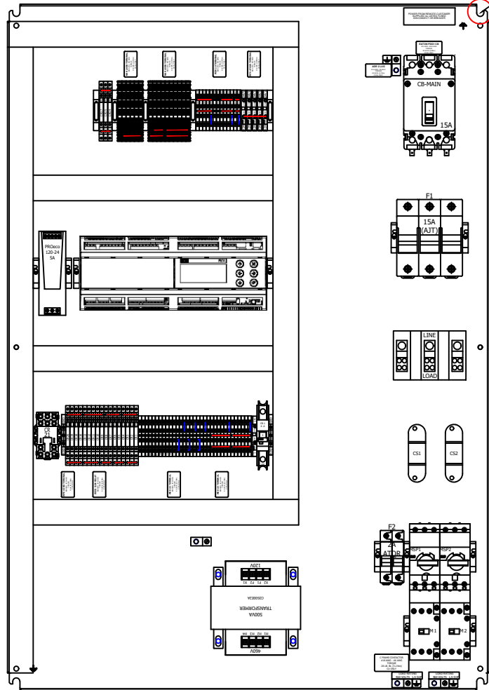
SUBPLATE PAINTED WHITE 40.2"(H) X 28.2"(W)
